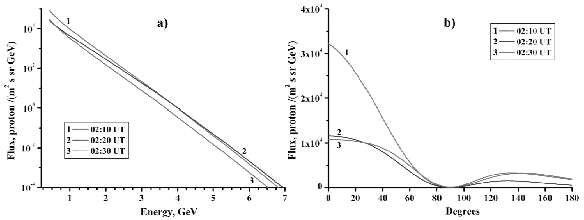
Fig. 1 a) Derived spectra of RSP; b) Pitch-angle distribution for the three moments of time.
