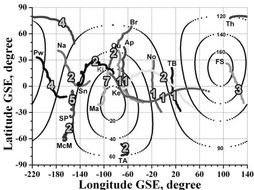
Fig. 3 GLE71. Asymptotic cones of some stations. Pw - Peawanuck, Na - Nain, SP - South Pole, McM - McMurdo, Sn - SANAE, Ki - Kiel, Ma - Mawson, Ou - Oulu, Ap - Apatity, Ke - Kerguelen, Br - Barentsburg, TA - Terre Adelie, No - Norilsk, TB - Tixie Bay, FS - Fort Smith, Th - Thule. Black dot lines are isogons with its pitch angle values. Bold green numbers on the cones indicate increase magnitudes of corresponding stations. The numbers are set at station sensitivity maxima to the derived spectrum at 02:20 UT. Distribution of these numbers along the map has a gap at \sim 90^\circ pitch angles.
