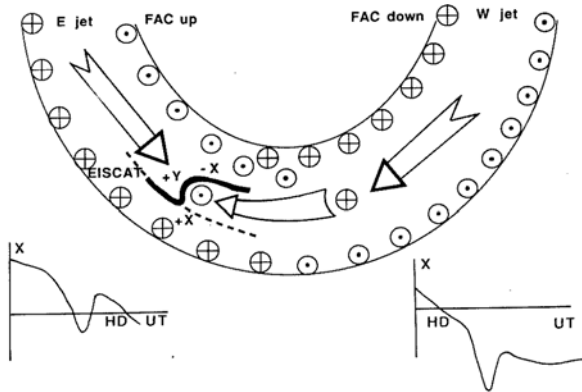
Figure 3: A schematic of superposition of the 3D systems for the global auroral currents and the substorm J_W .
