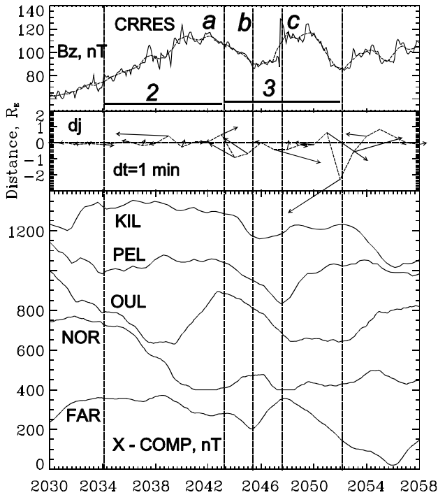
Figure 5: Substorm on March 12, 1991, intensifications 2 and 3.
