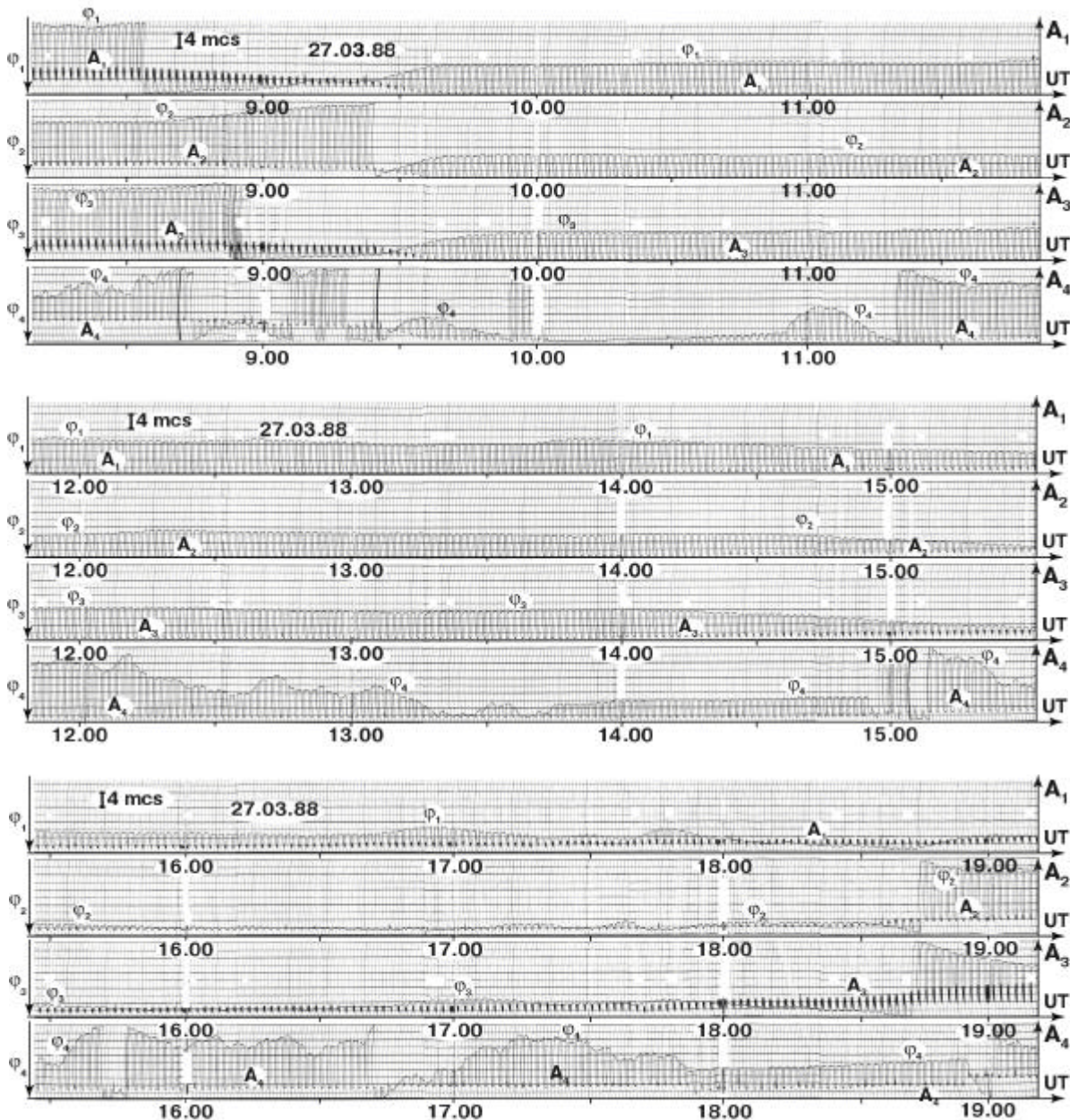
Fig. 1. The example of the VLF variations during UrEP
